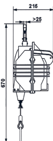
Balancer 169361-169369
